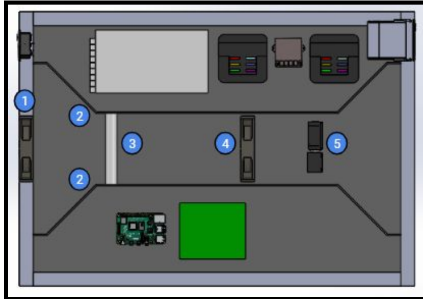
Figure 6: Bottom side of the metal base. 1. Intake air fan 2. Air duct walls 3. PVC pipe 4. Circulation fan 5. 100 W and 200 W heaters. The rest are electrical and computer components.
