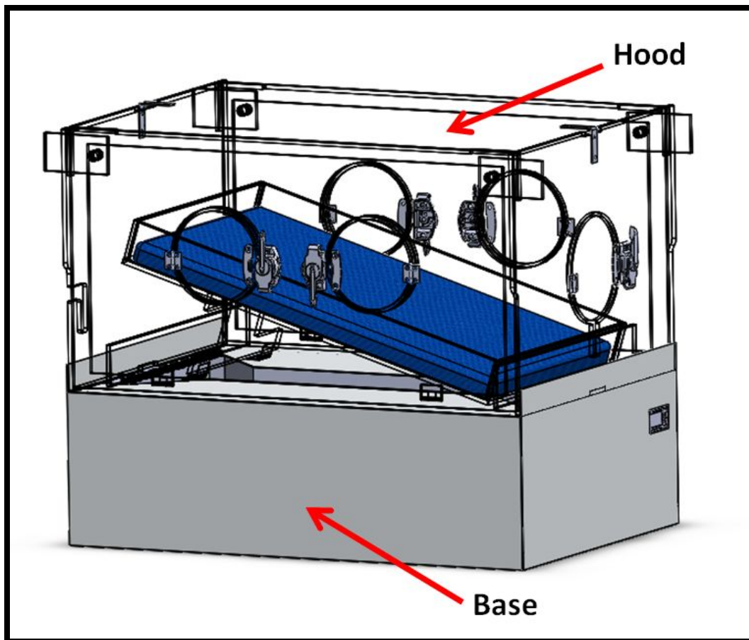
Figure 3: The final concept design for the entire incubator including the base and the hood.
