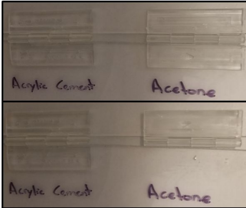
Figure 10: This shows the results of the rapid prototype of the acrylic cement vs. the acetone as a method of adhesion for the acrylic hinges. The top image shows both were set up the same way to connect two sheets of acrylic and the bottom image shows the results after 3 days of letting them dry where the acetone prototype broke off of one side.
