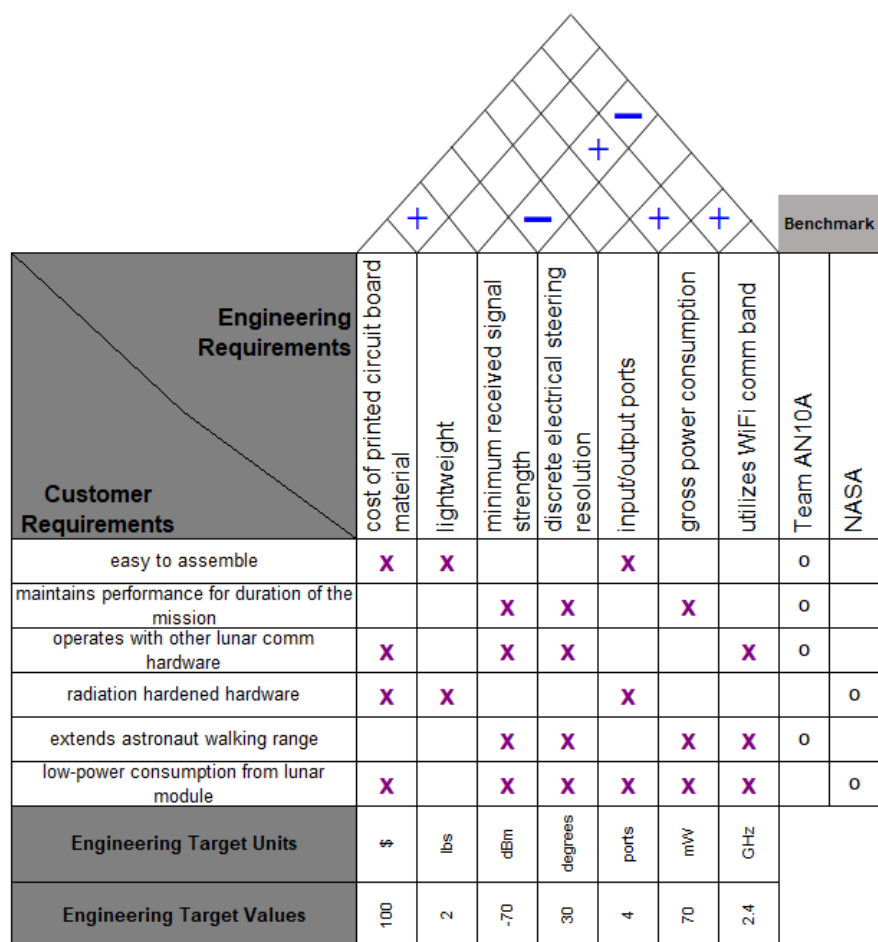
Figure 1. QFD chart for team AN10A's phased array antenna system
