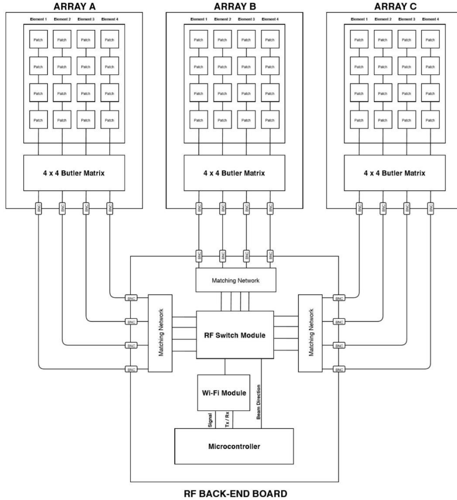
Figure 2. System-level architecture for the proposed phased array system
