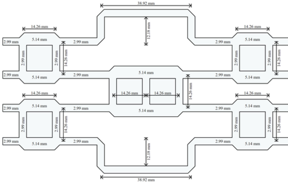
Figure 4. Butler matrix topology and dimensions for a 4x4 phased array operating at 2.4 GHz
