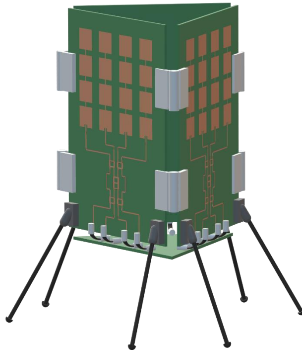
Figure 5. 3D model of system, showing arrangement of array panels and back-end board
