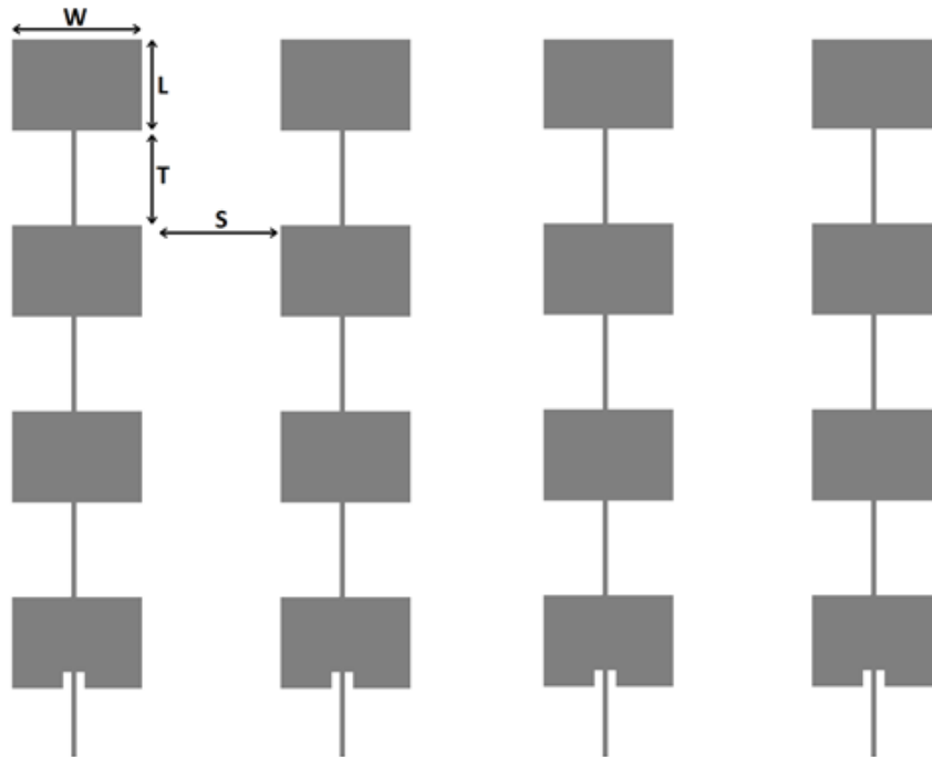
Figure 3. 4x4 linear antenna array comprised of stacked microstrip patch antennas
